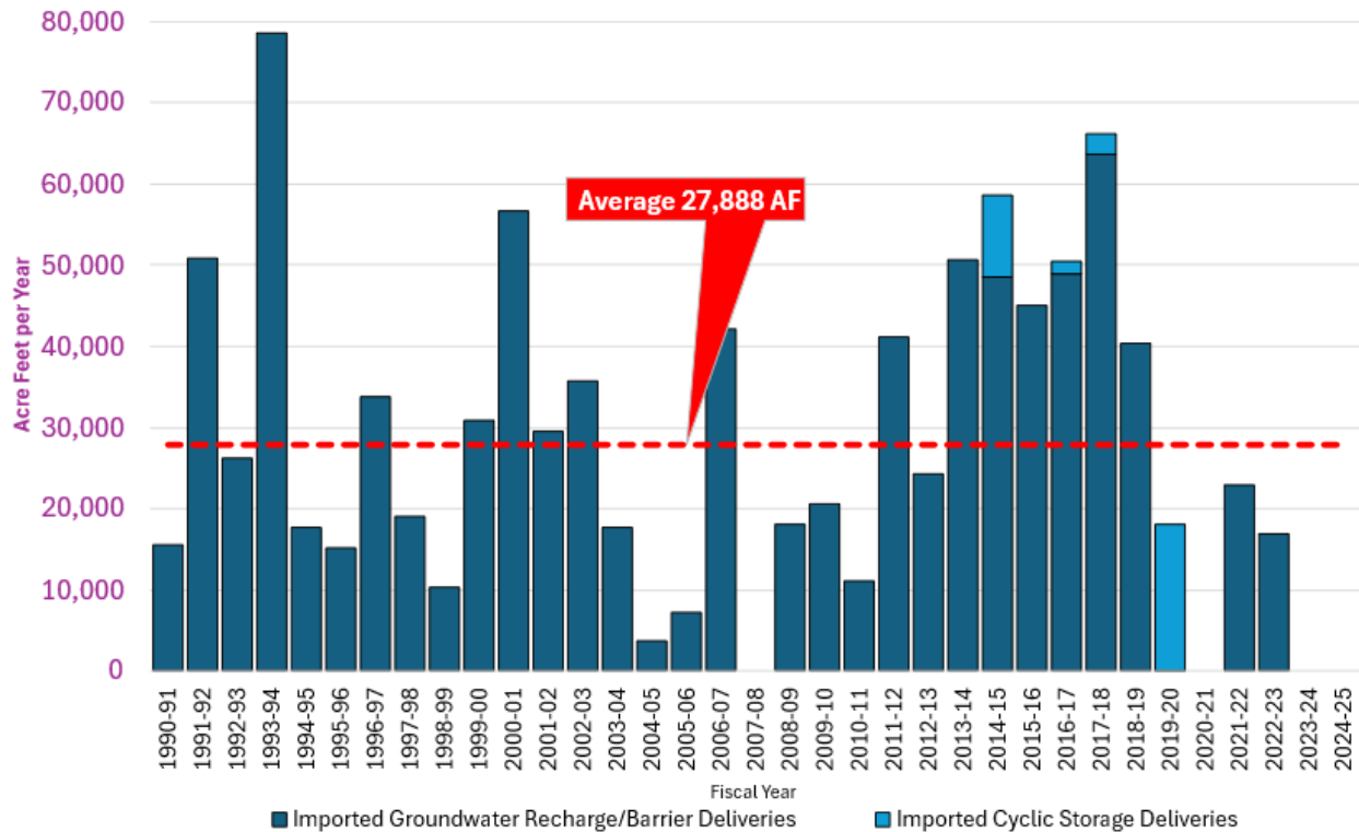
Figure 6.6 MWD Imported Water Sales for Groundwater Replenishment
