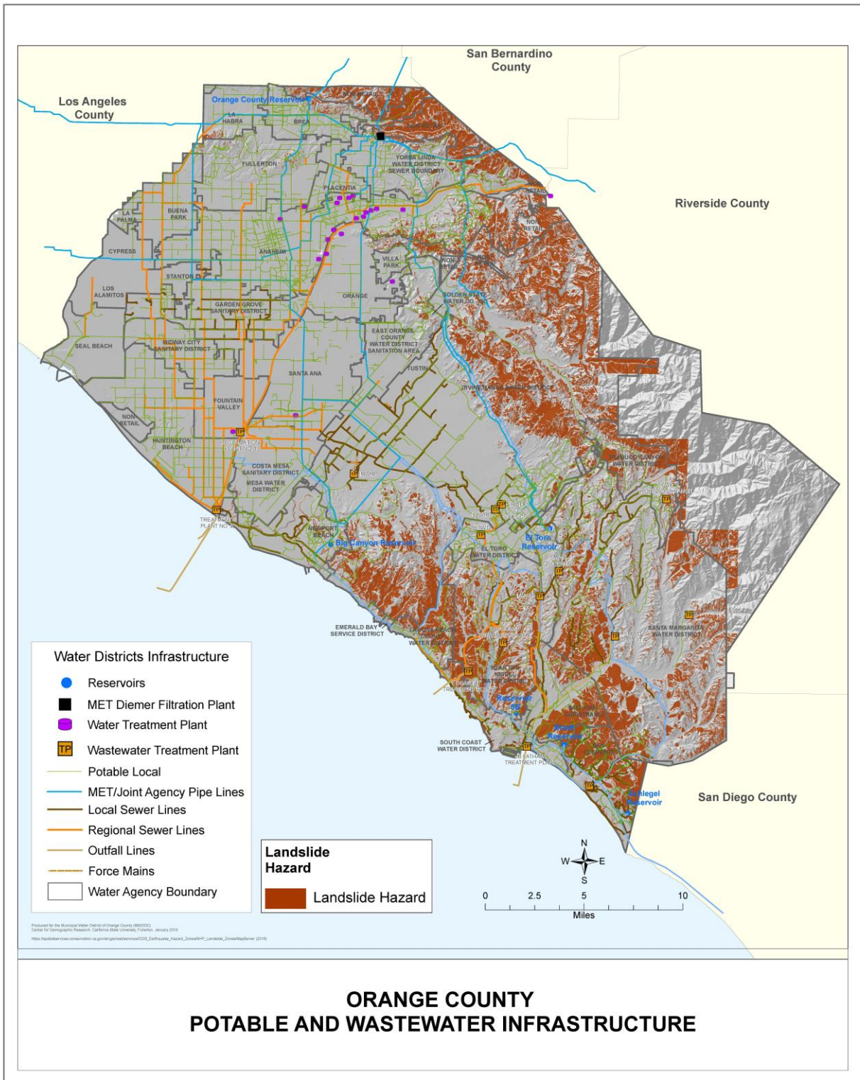
Figure 3-10 Landslide Susceptibility
